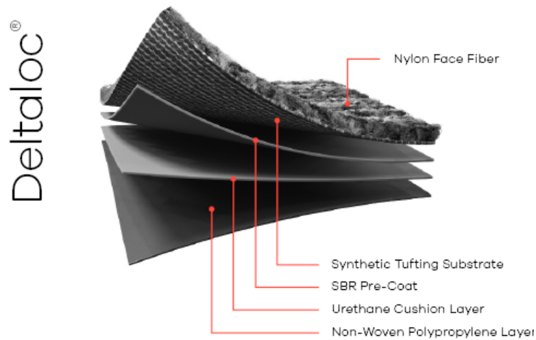
Figure 1: Product Construction
