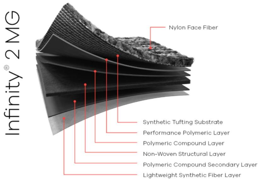
Figure 1: Product Construction
