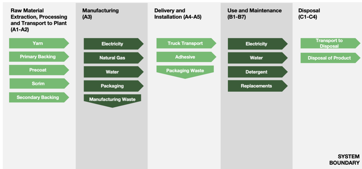
Figure 3: System Boundary
