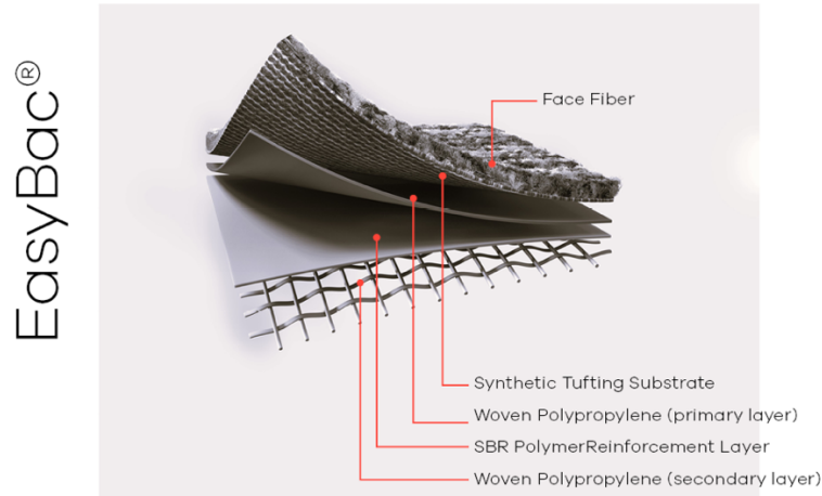
Figure 1: Product Construction
